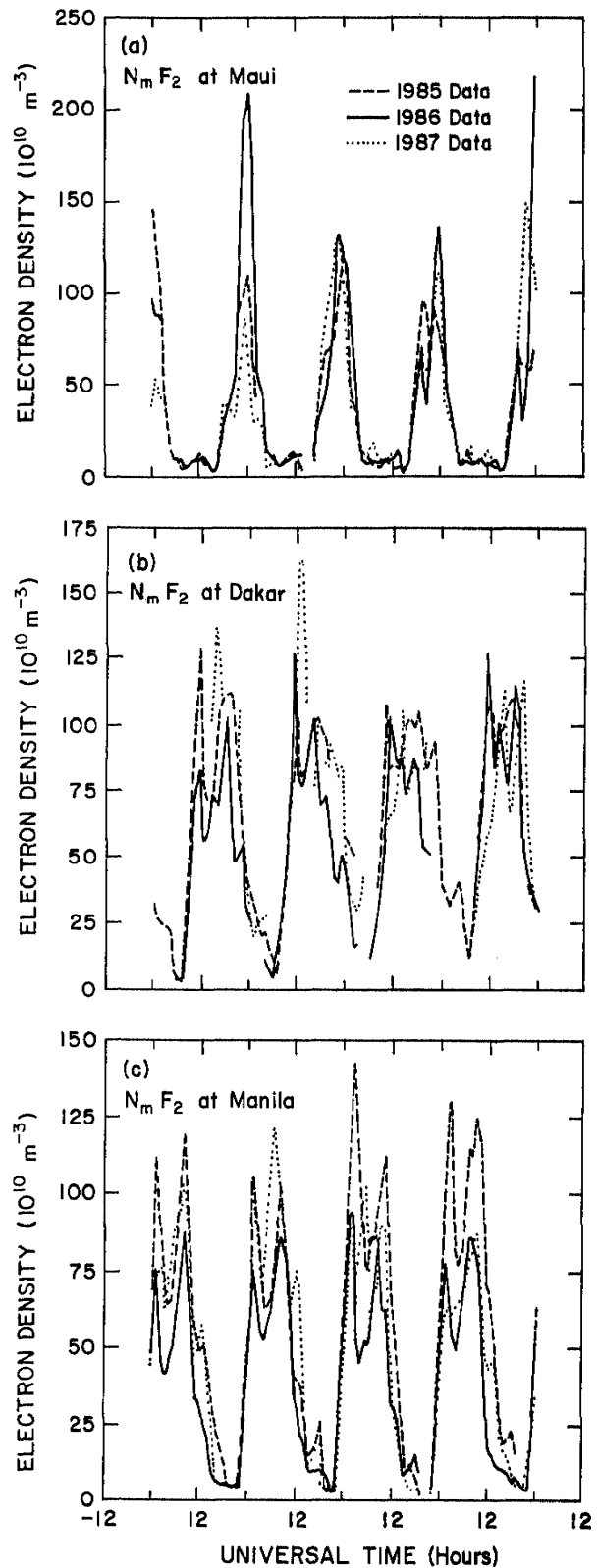
Fig. 6. Ionosonde measurements of N_m F_2 over (a) Maui ( 20^\circ N ), (b) Dakar ( 15^\circ N ), and (c) Manila ( 15^\circ N ) during January 14-17, 1985 (dashes), January 14-17, 1986 (solid), and January 27-30, 1987 (dots).
